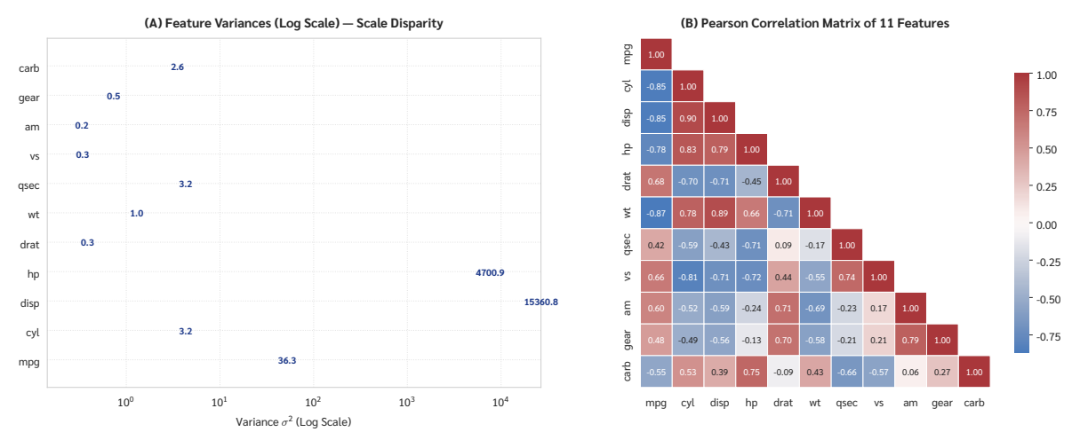
Figure 3: MTCARS Exploratory Data Analysis — Variance Discrepancy & Feature Interrelations
